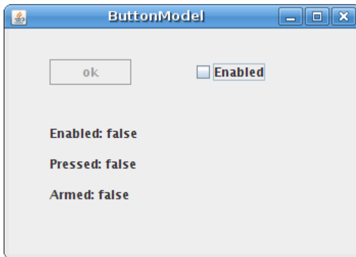
Figure: ButtonModel
