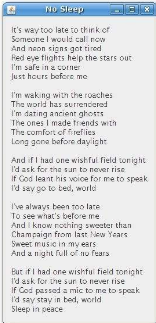
Figure: JLabel
