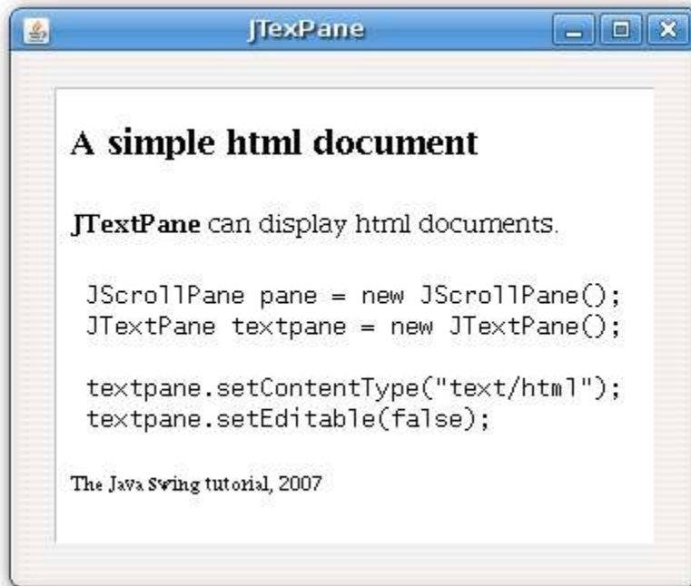
Figure: JTextPane
