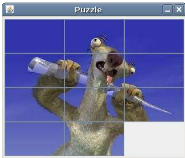
Figure: Puzzle
