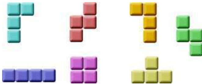
Figure: Tetrominoes
