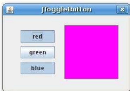
Figure: JToggleButton
