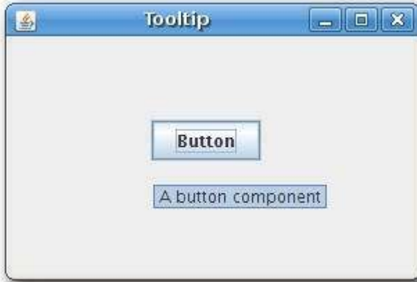
Figure: Tooltip
