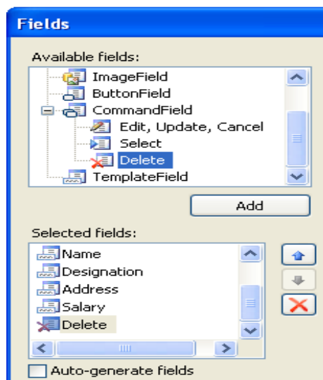
Figure 3.4-4: Adding Delete link through CommandField in Field Colums.
