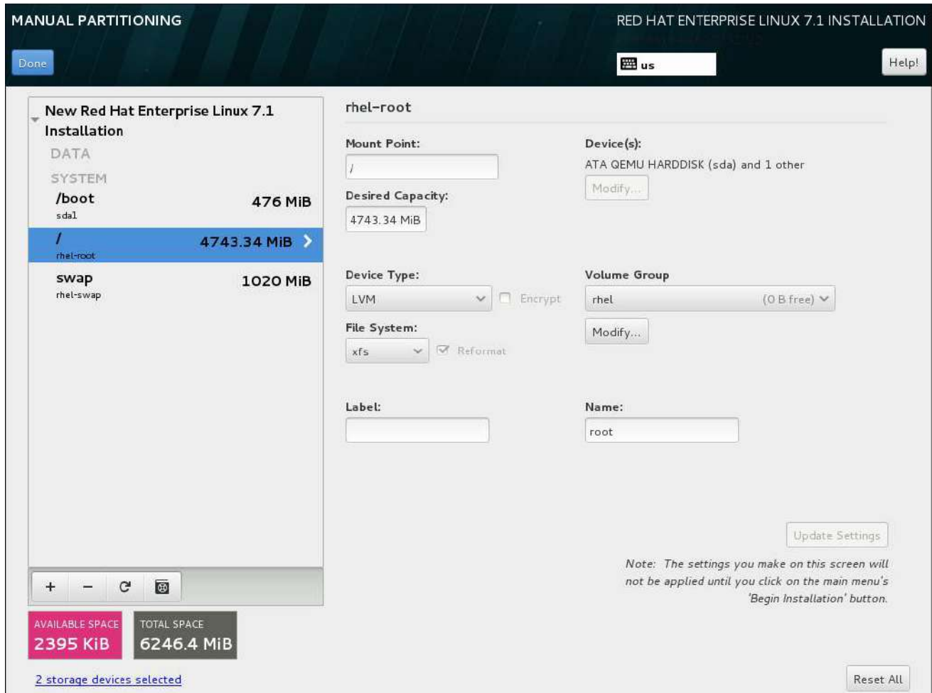
Figure 8.25. Customizing Partitions
