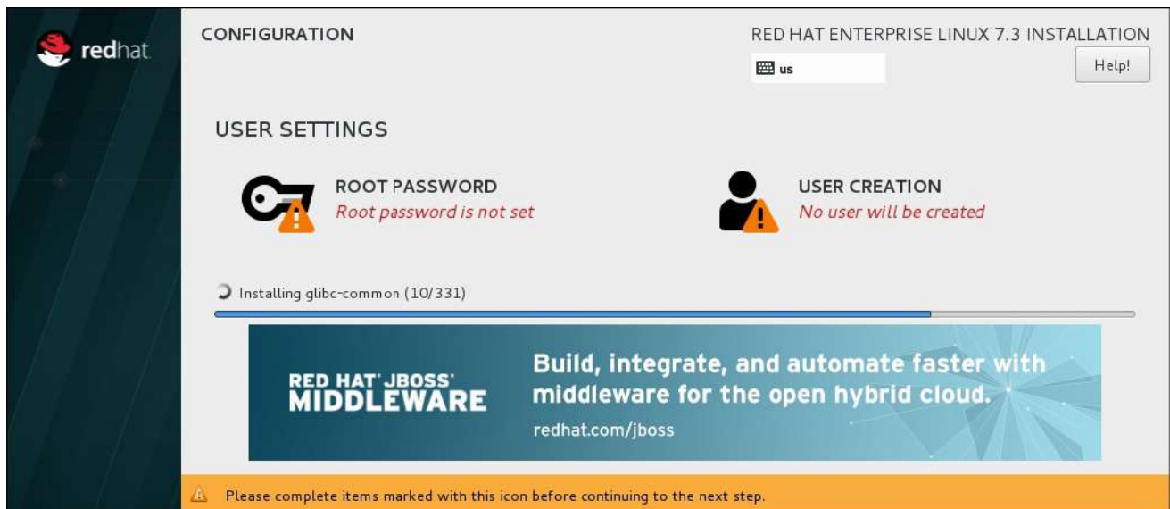
Figure 17.38. Installing Packages
