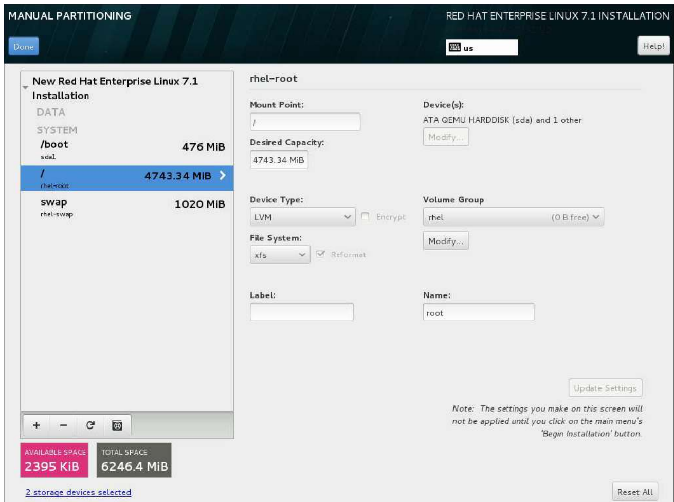
Figure 17.22. Customizing Partitions
