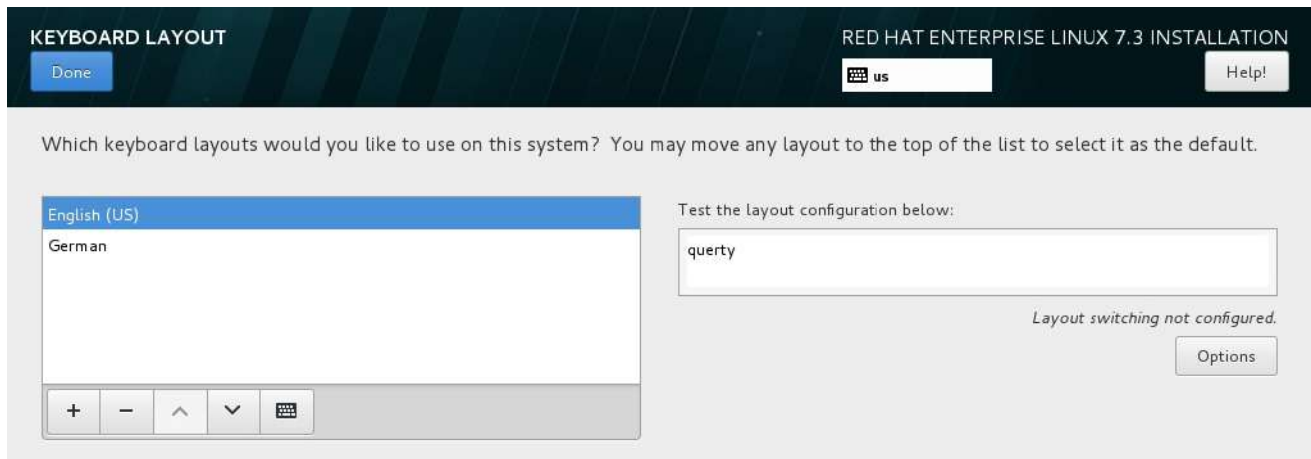
Figure 17.7. Keyboard Configuration
