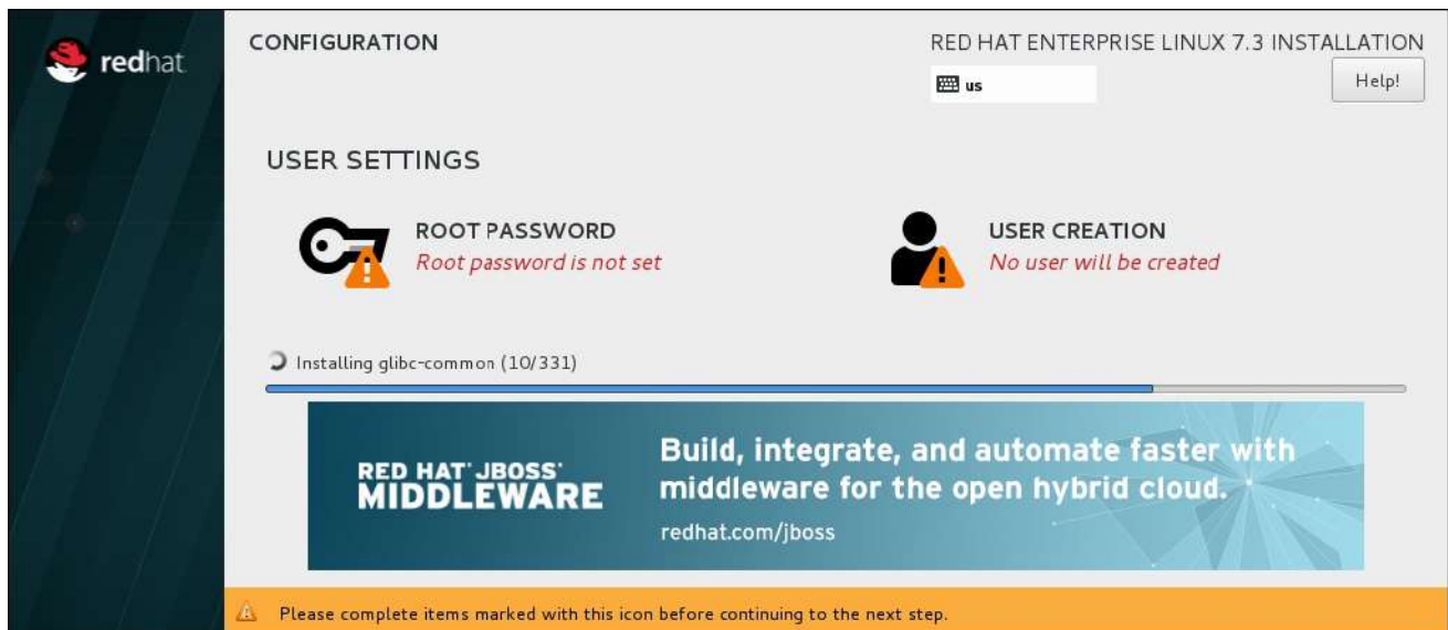
Figure 8.38. Installing Packages
