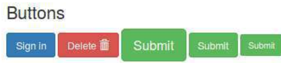
Fig. 3.6: Buttons
