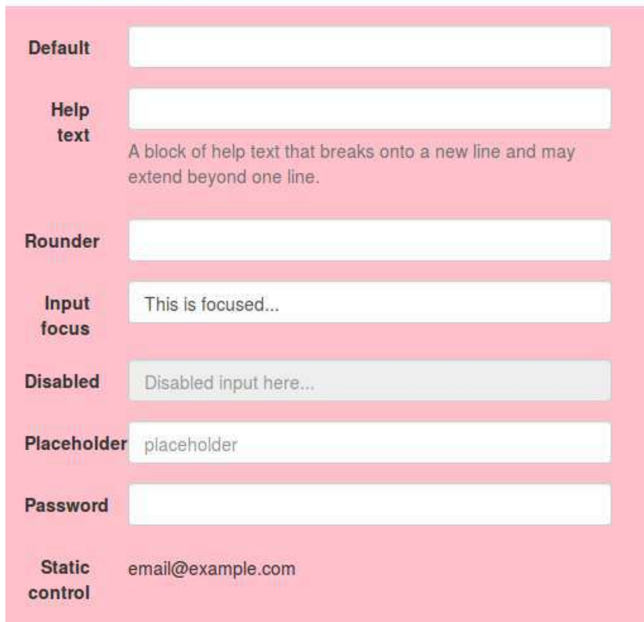
Fig. 3.11: Form elements
