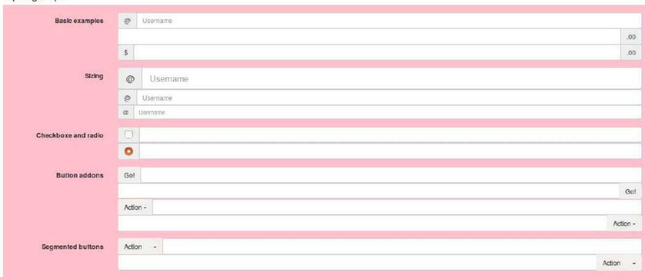
Fig. 3.14: Input groups
