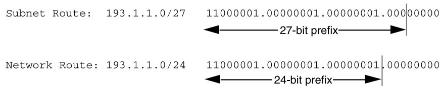
FIGURE 13. Differentiating Between a Route to the All-0s Subnet and the Entire Network
